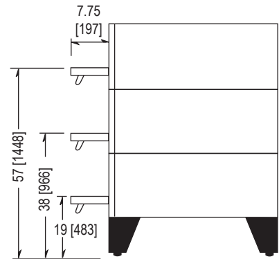
SIDE VIEW - EDO 2136 Triple
