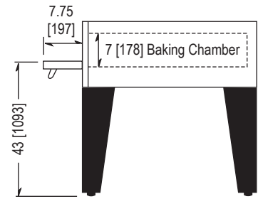
SIDE VIEW - EDO 2136 Single
