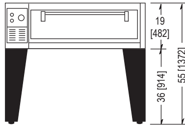
SIDE VIEW - EDO 2136 Single
