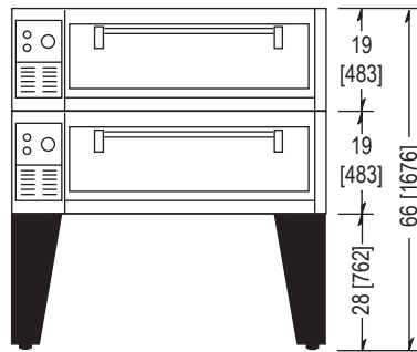
SIDE VIEW - EDO 2136 Double
