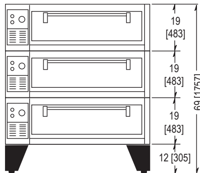
SIDE VIEW - EDO 2136 Triple
